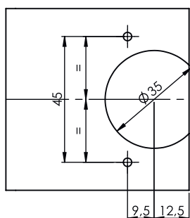
Foratura anta Door Drilling
