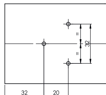
Foratura fianco Side Drilling
