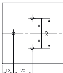
Foratura fianco Side Drilling
