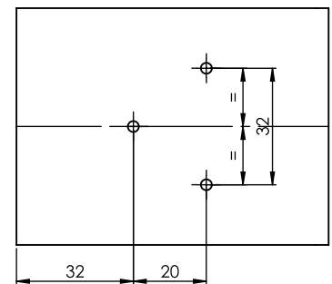
Foratura fianco Side Drilling
