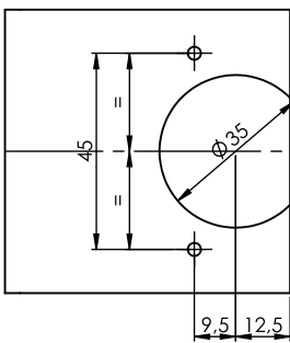
Foratura anta Door Drilling
