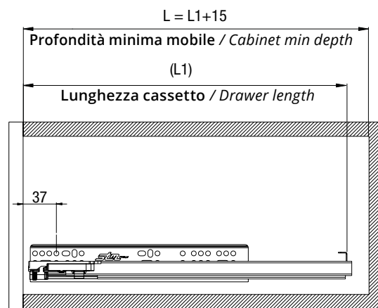
Cassetto standard / Standard drawer
