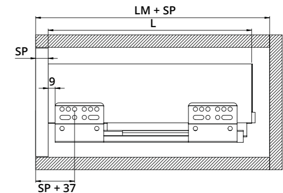
Foratura fianco con frontale interno Side panel hole drilling with inner drawer front
