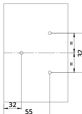
Foratura fianco Side Drilling
